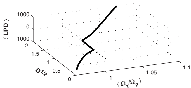
FIG. 4. \langle \text{LPD} \rangle as a function of noise intensity \sqrt{D} and the mean coupling frequency ratio \langle \Omega_1/\Omega_2 \rangle . The values for noise variances are \sigma_1^2=0.003 and \sigma_2^2=0.0003 , and for the coupling strength \beta=166 .
